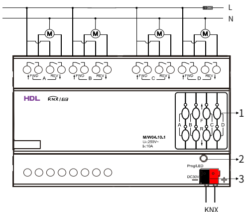
Figure 4. Wiring
