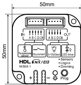
Figure 2. Dimensions-Front View
